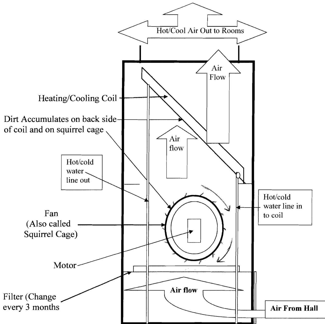
Typical Heating/Cooling Unit.
